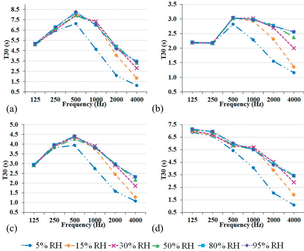
Figure 13. Post-tuning (p) T30 results under different relative humidity levels (RH) (a: YK, b: KM, c: KY, d: TA).
