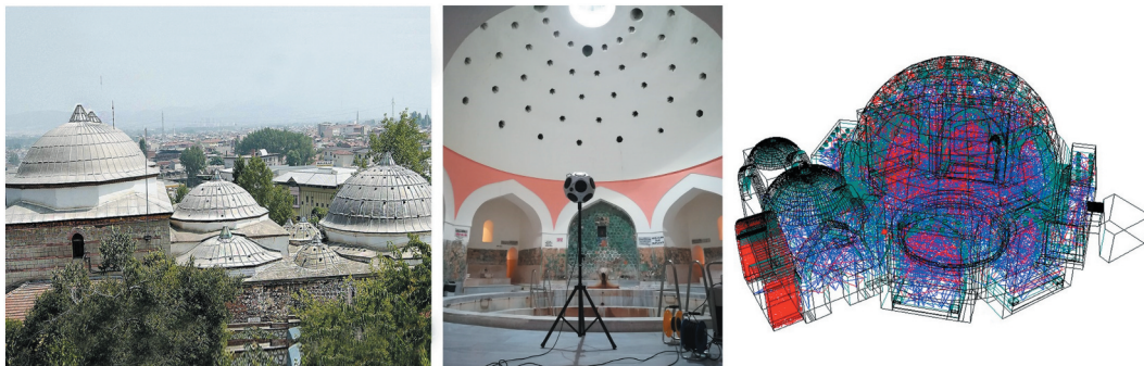
Figure 2. Yeni Kaplıca, exterior view (left), interior view (middle) measurement set-up, ray tracing model of caldarium (right).
