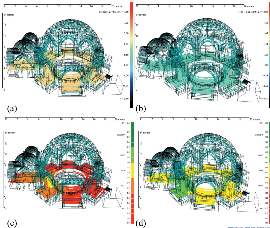
Figure 11. T30 and STI Distribution maps for Yeni Kaplıca (YK) caldarium section: (a) post-tuning (p) scenario T30 distribution map for 1000 Hz; (b) historical plaster (hp) scenario T30 distribution map for 1000 Hz; (c) post-tuning scenario (p) STI distribution map; and (d) historical plaster scenario (hp) STI distribution map.
