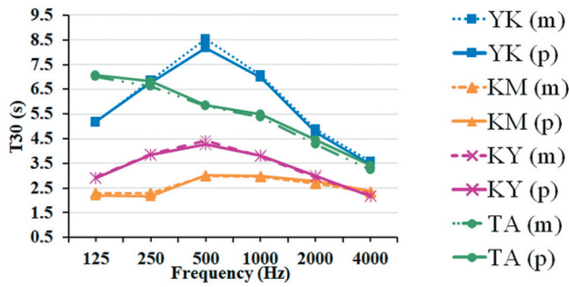
Figure 10. Measurement (m) and post-tuning (p) results for all four caldaria, over 1/1 octave bands.
