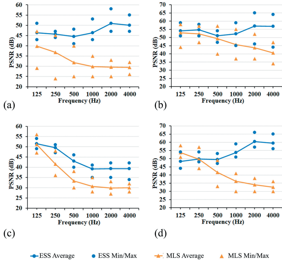
Figure 8. Comparison of INR over 1/1 octave bands in Hz (a:YK, b:KM, c:KY, d:TA).
