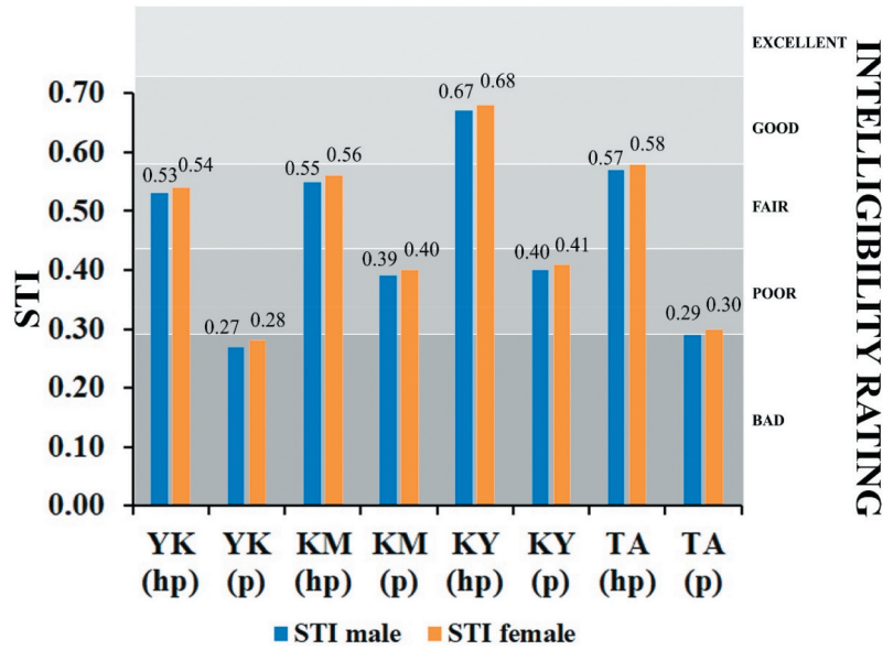
Figure 14. Male and female STI results for all four caldaria, post-tuning scenario (p) vs. historical plaster scenario (hp).
