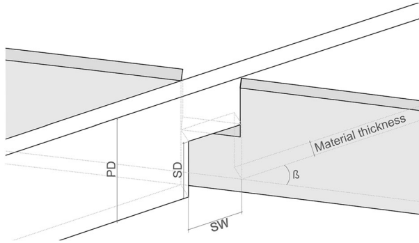
Fig. 9 Slit formation detail
